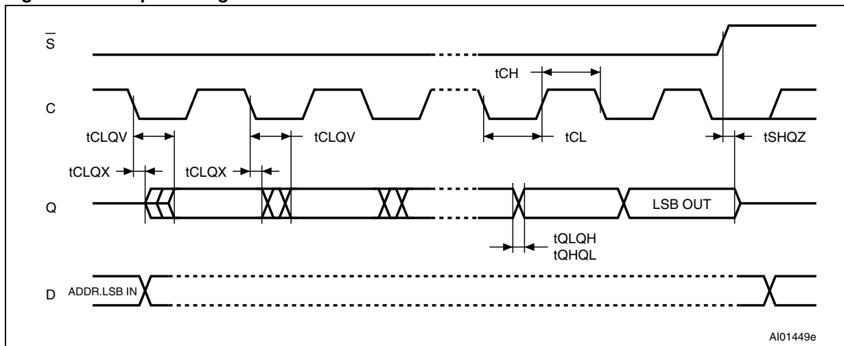
Figure 18. Output timing
